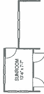
PARTIAL PLAN W/ OPT. SUNROOM
