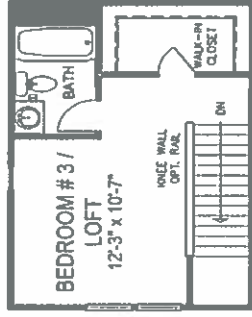
PARTIAL PLAN W/ OPT. FINISHED LOFT
